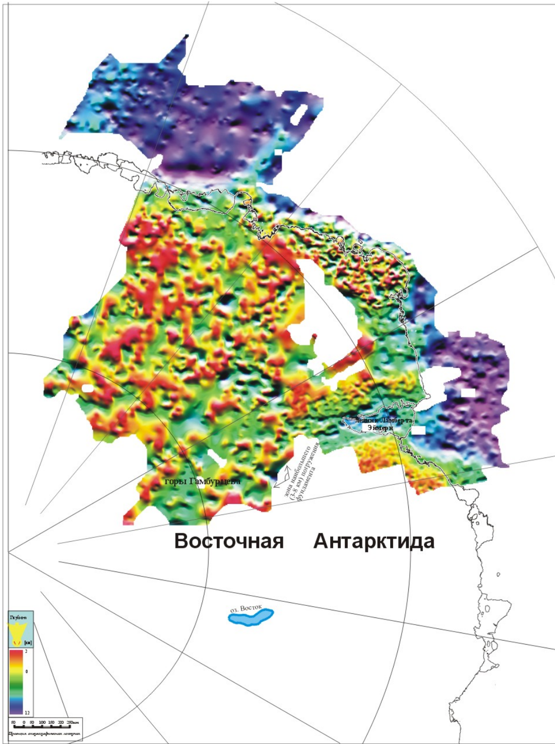
Map of magnetic active basement surface
